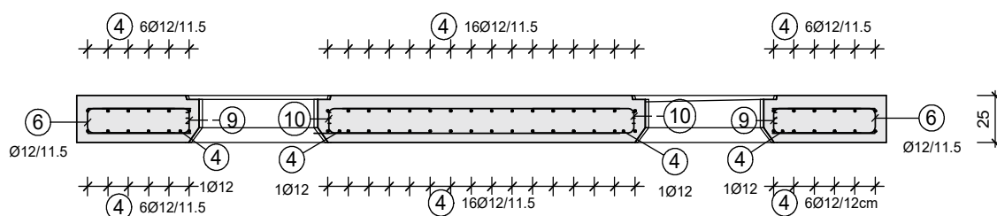
Cut 3 - 3
