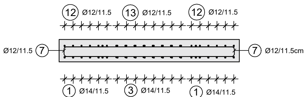
Cut 2 - 2
