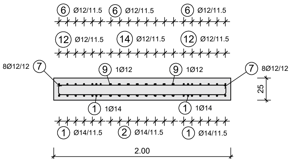
Cut 1 - 1
