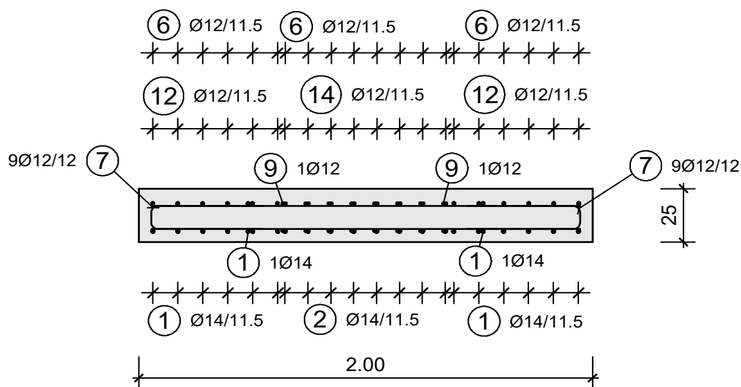
Cut 1 - 1
